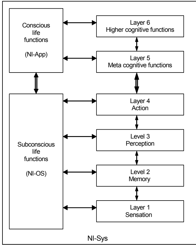
Fig. 1. The layered reference model of the brain (LRMB)
