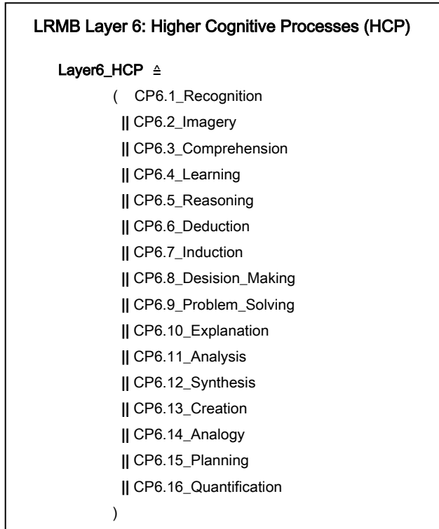
Fig. 6. Cognitive processes at the higher cognitive functions layer of LRMB
