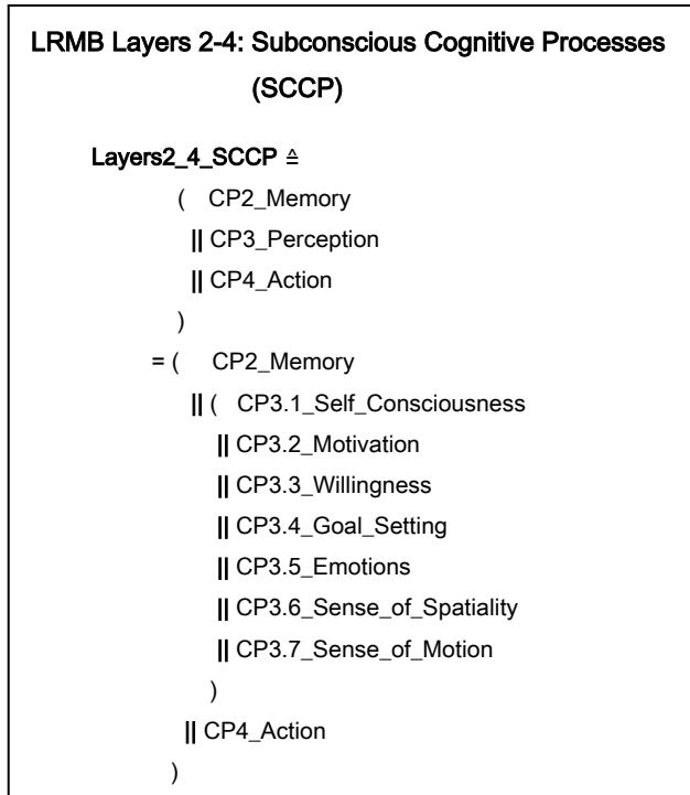
Fig. 4. Cognitive Processes at the subconscious layers of LRMB
